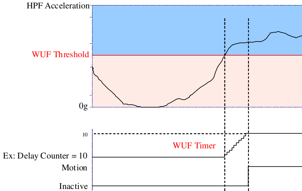
Figure 3. Latched Motion Interrupt Response
